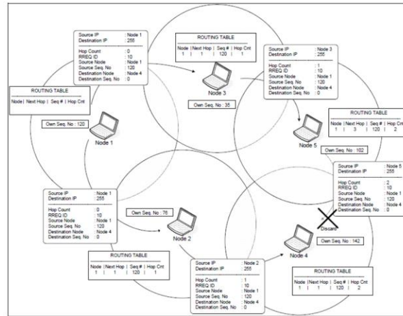
Fig 3.1 - Propagation of the RREQ message
