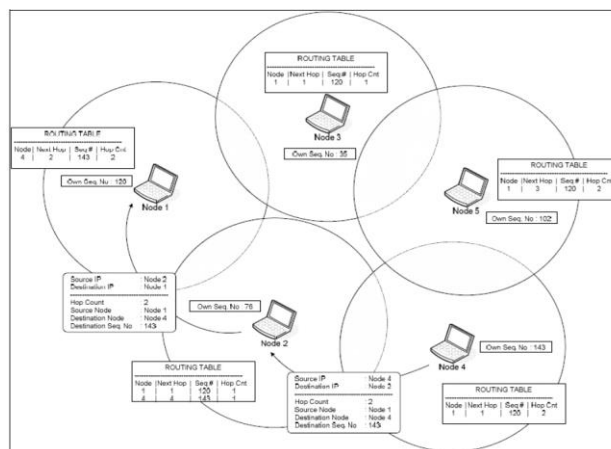
Fig 3.2 - Unicasting the RREP message
